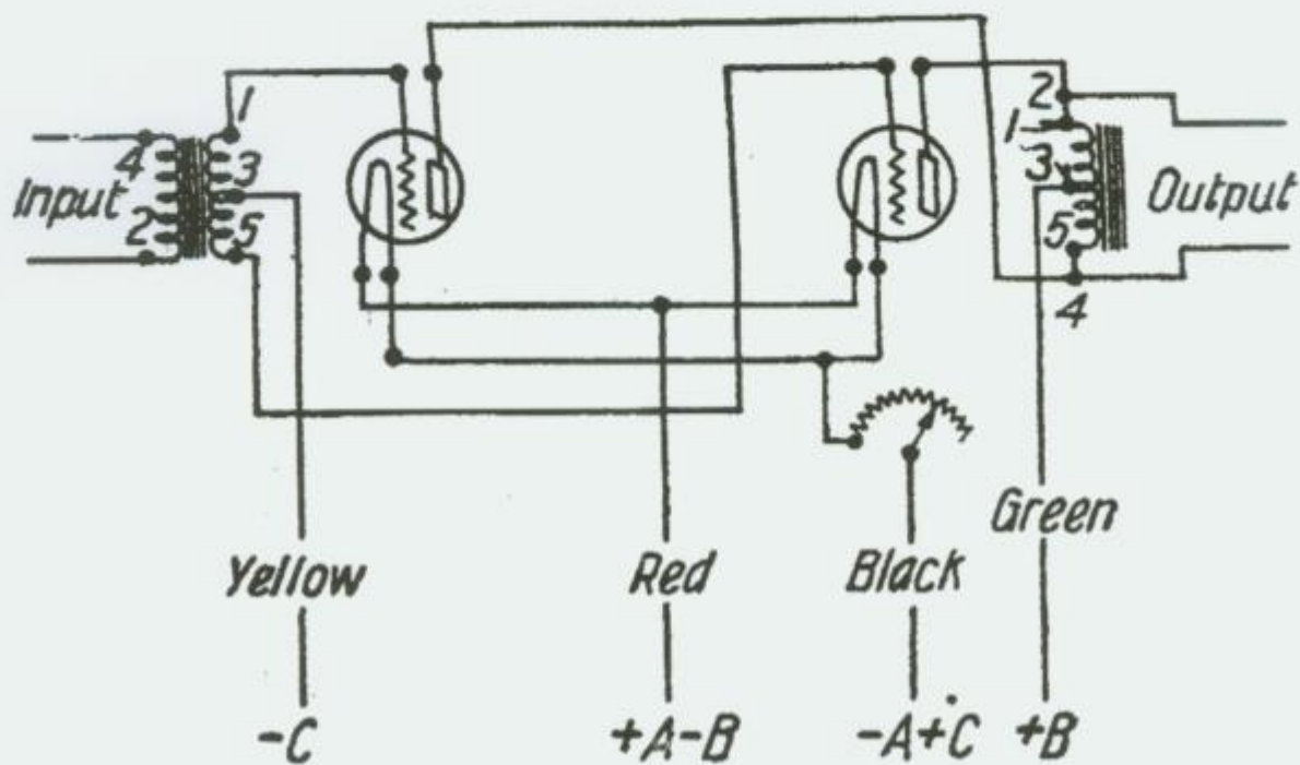
Fig. 2—Diagram of Connections
