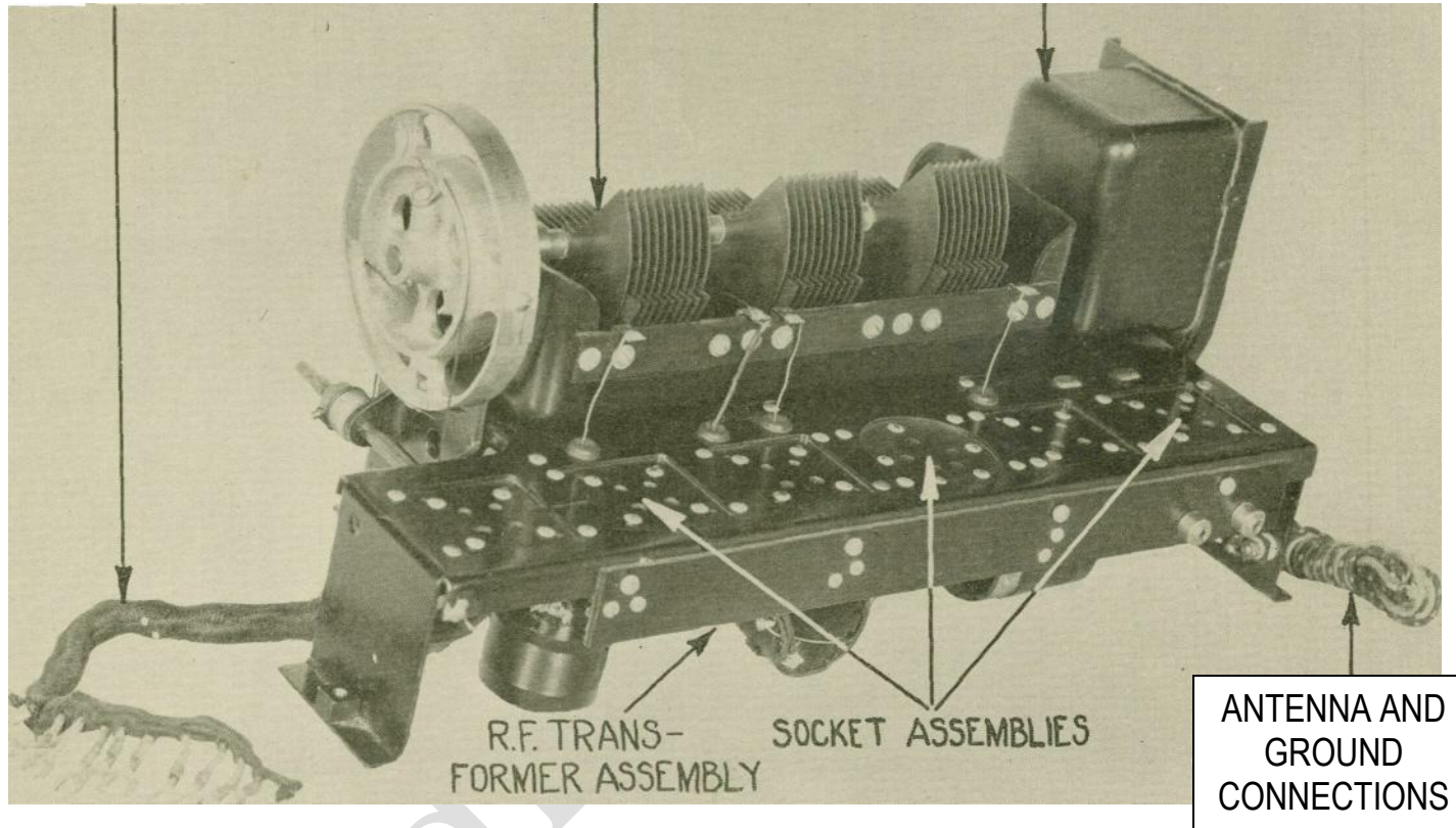
Figure 1—Top view of chassis assembly showing the principal parts.
