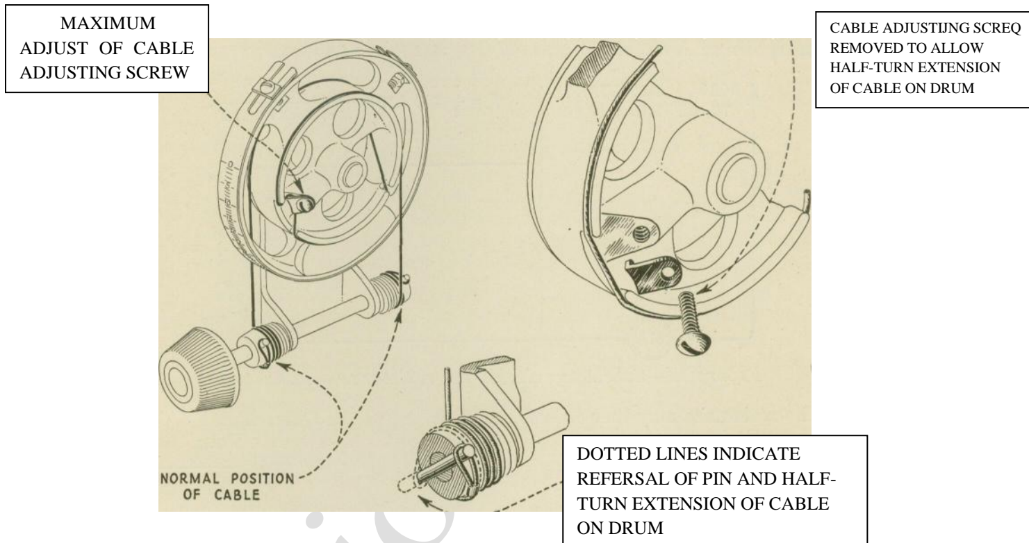
Figure 10—Radiola 17 three-gang condenser cable and drum operating mechanism.
