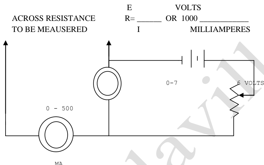
Figure 12—Schematic circuit for resistance measurement.
