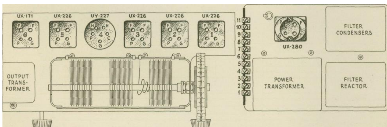
Figure 5—Radiotron socket contacts
