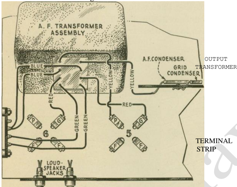
Figure 22—Detail of A. F. transformer connections and color scheme of wiring.
