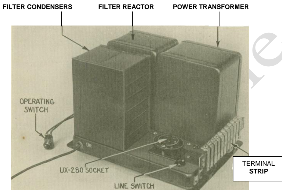
Figure 2—Socket Power Unit showing various parts.
