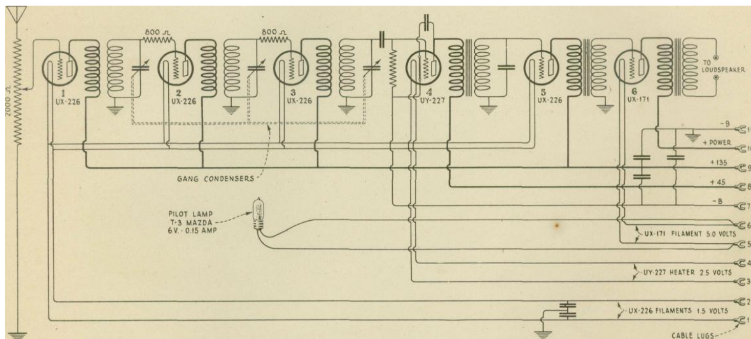
Figure 4—Schematic circuit diagram of receiver assembly.
