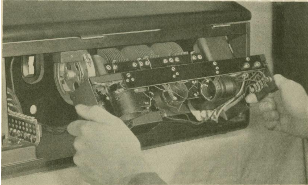
Figure 19—Removing the receiver assembly from the cabinet.
