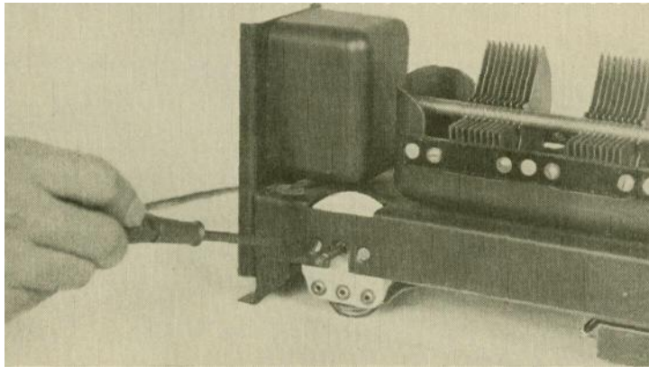
Figure 7—Releasing mounting screws holding volume control.
