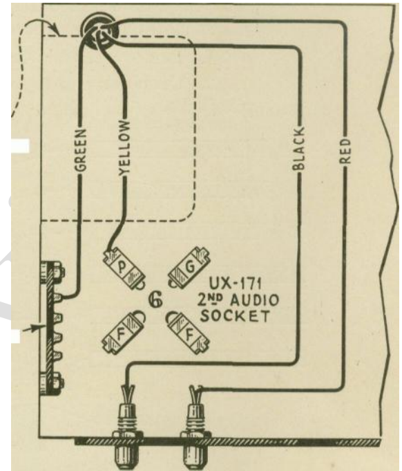
F Figure 23—Output transformer connections.
