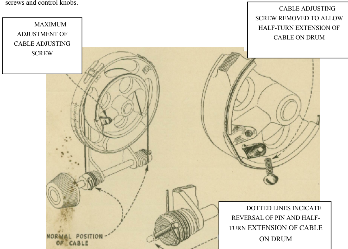
Figure 4—Three-gang condenser cable and drum operating mechanism
