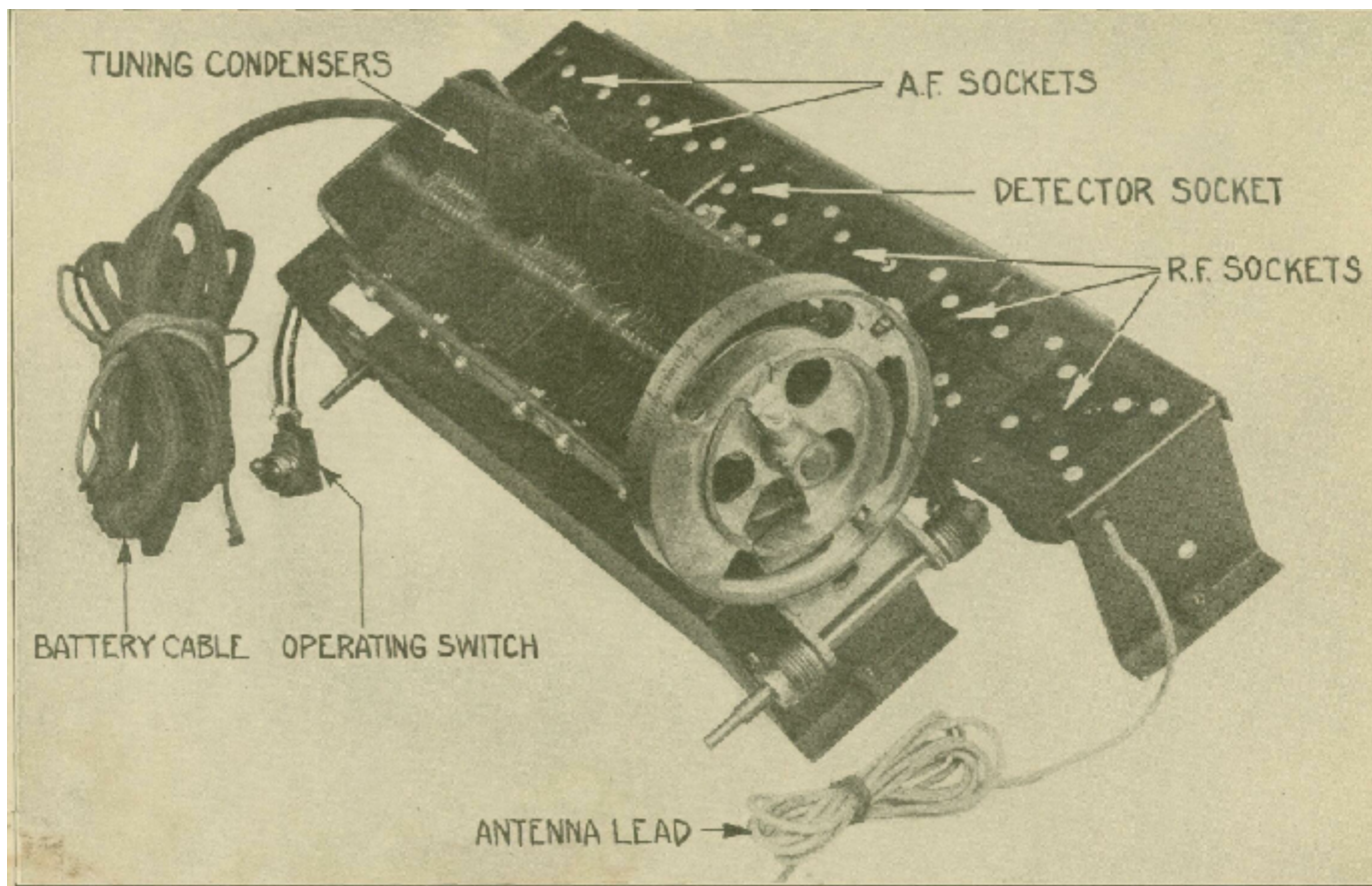
Figure 1—Top view of chassis showing the simple arrangement and rugged construction of the three-gang condensers, gang sockets and tuning control.
