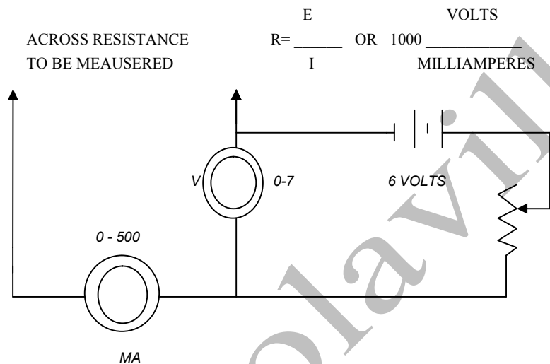
Figure 6—Schematic circuit for resistance measurement
