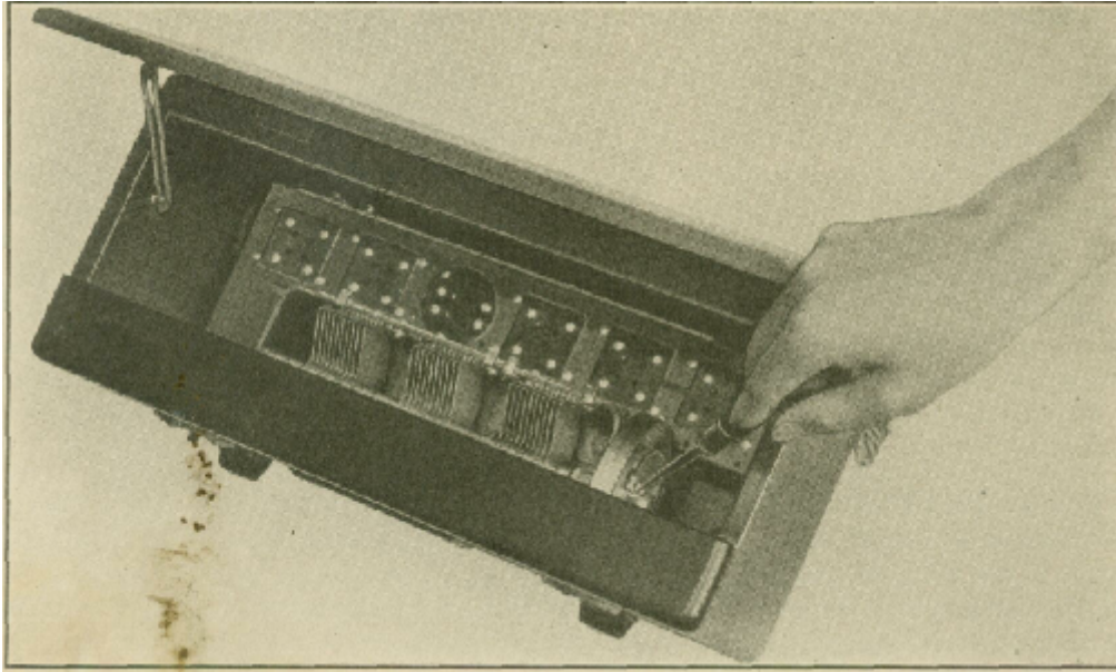
Figure 3—Timing the cable adjusting screw to take up slack in condenser control cable
