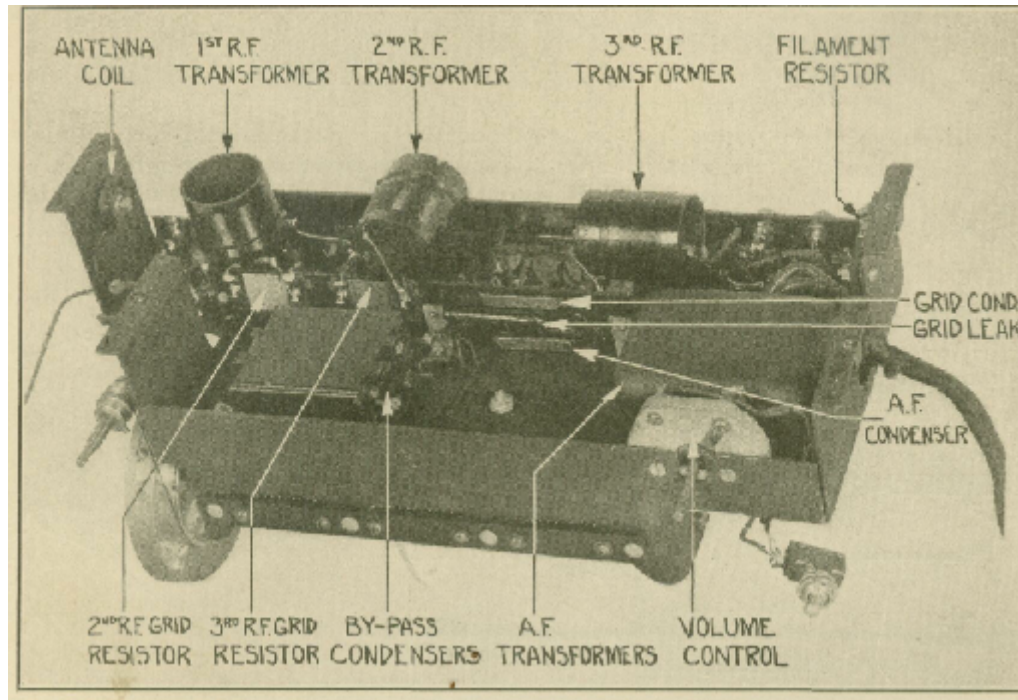
Figure 9 —Sub-chassis assembly showing antenna coil, radio frequency coils, by-pass condensers, resistances and audio frequency transformers
