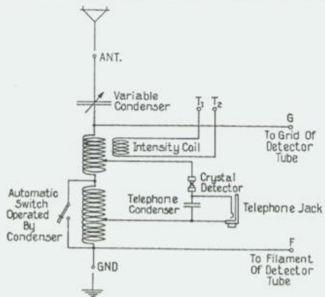
Connection Diagram
